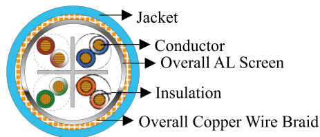
Cat6A SF/UTP
